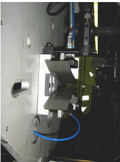
Low pressure gluing station installed on a flexo folder-gluer machine
